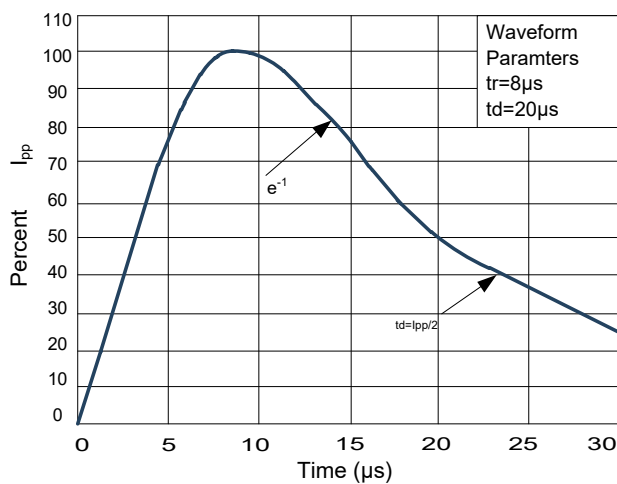
Figure3: Pulse Waveform
